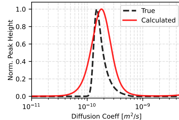
S5 (Xu) - 1D Distribution
