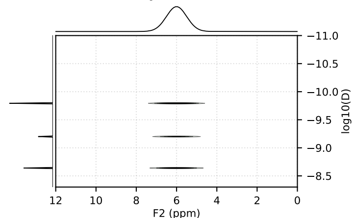
S3 (Sparse) - 1D Distribution
