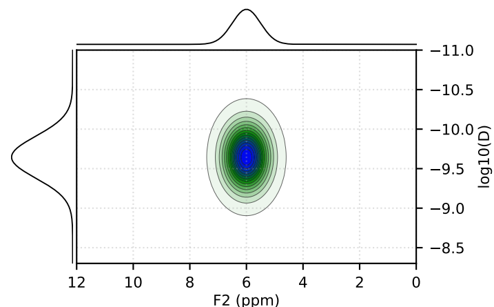
S4 (Gauss) - 1D Distribution
