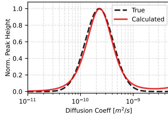
S4 (Gauss) - 1D Distribution
