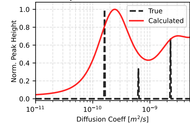
S3 (Sparse) - 1D Distribution
